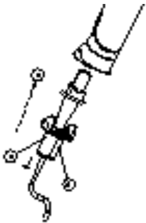
Pull the cable downwards until the top of the clamp meets the widest part of the cable.
